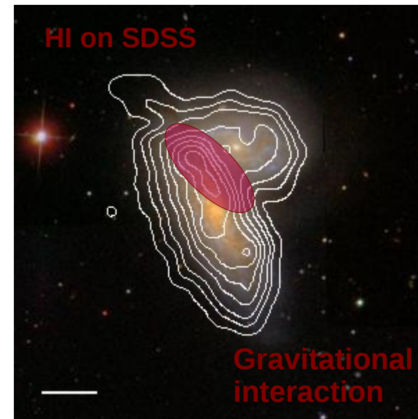
NGC 4567/68
